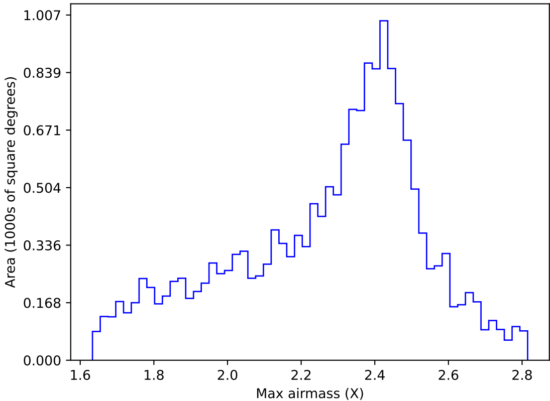
ddf_acor_sf30_lsf40_lsr20_v3.4_10yrs WFD r band: Max airmass
