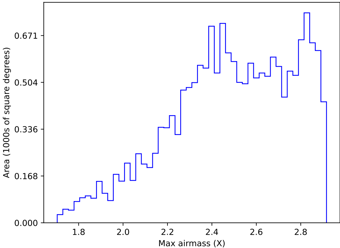
ddf_acor_sf30_lsf40_lsr20_v3.4_10yrs WFD i band: Max airmass
