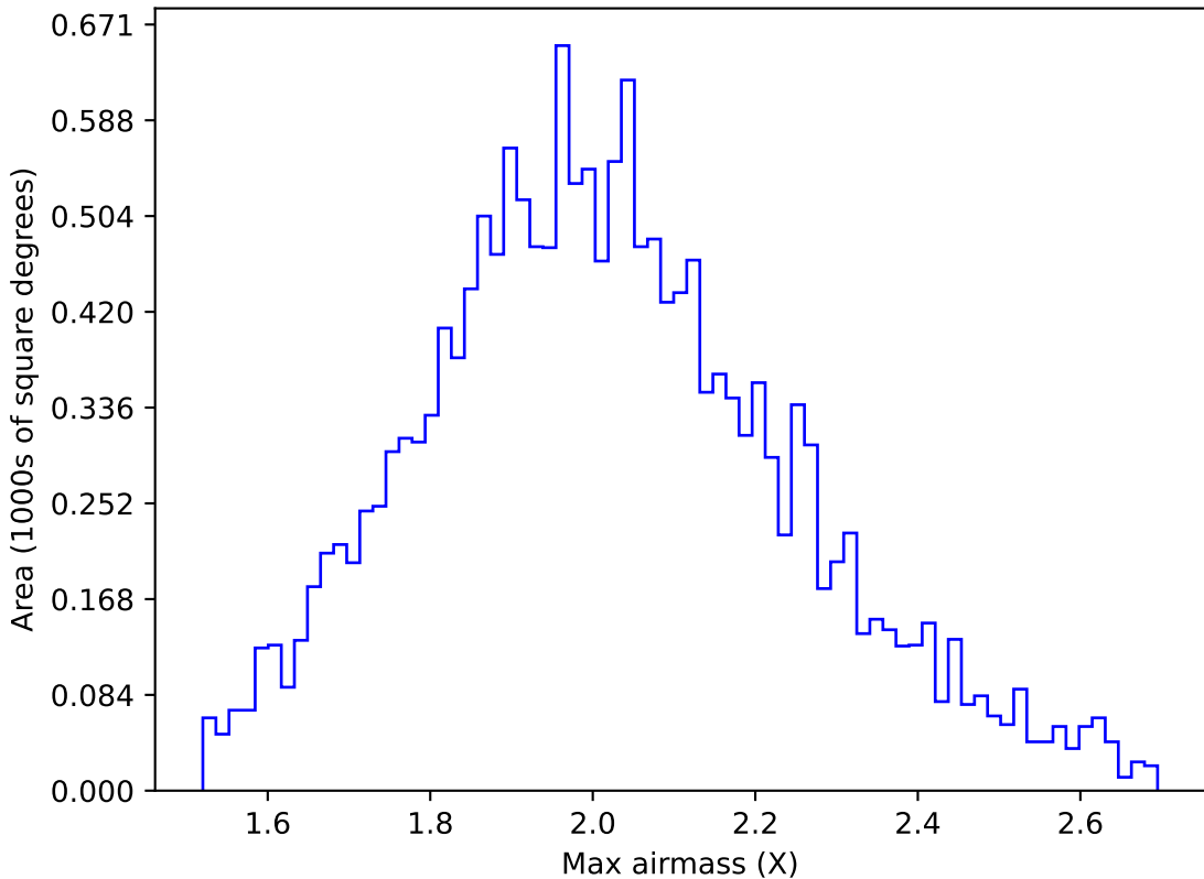
ddf_acor_sf30_ls40_lsr20_v3.4_10yrs WFD g band: Max airmass
