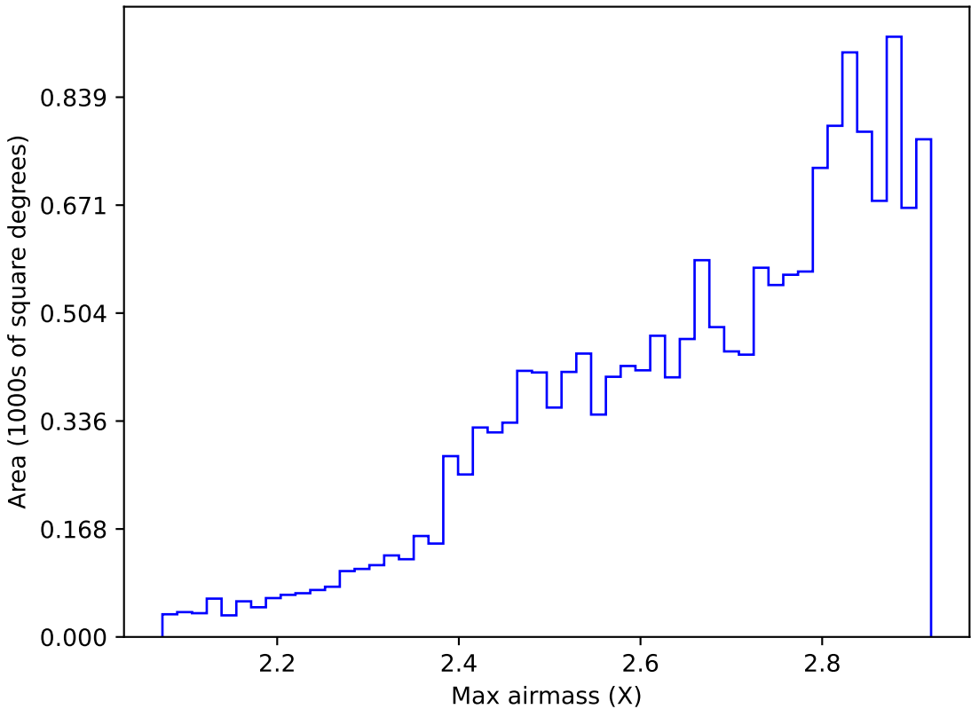
ddf_acor_sf30_lsf40_lsr20_v3.4_10yrs WFD all bands: Max airmass
