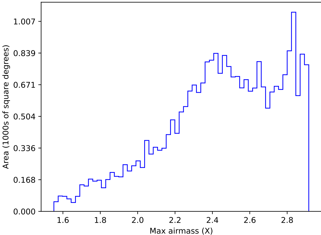
ddf_acor_sf30_lsf40_lsr20_v3.4_10yrs All sky z band: Max airmass
