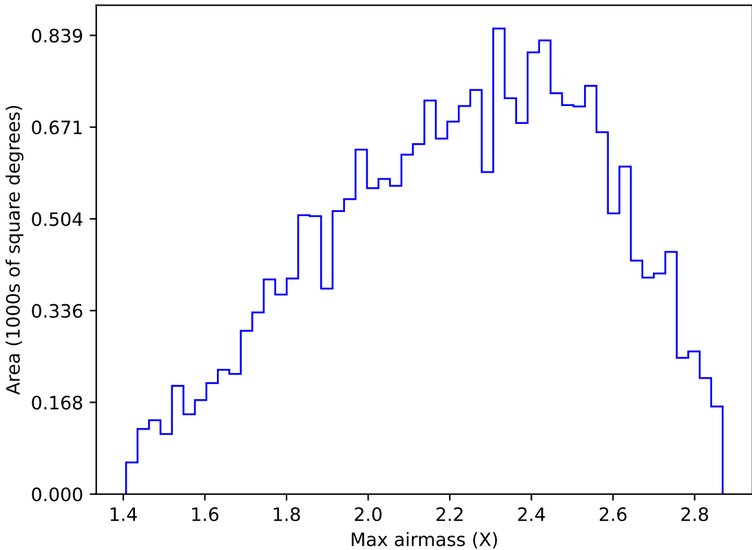
ddf_acor_sf30_lsf40_lsr20_v3.4_10yrs All sky y band: Max airmass
