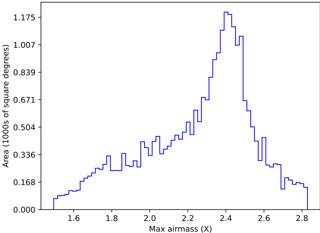
ddf_acor_sf30_lsf40_lsr20_v3.4_10yrs All sky r band: Max airmass
