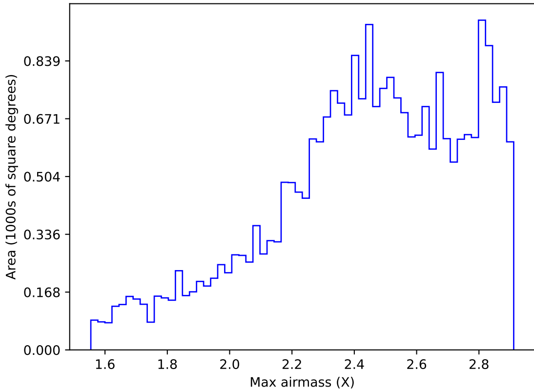
ddf_acor_sf30_lsf40_lsr20_v3.4_10yrs All sky i band: Max airmass
