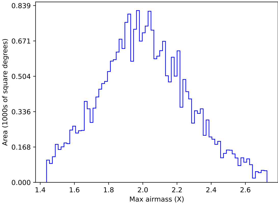
ddf_acor_sf30_lsf40_lsr20_v3.4_10yrs All sky g band: Max airmass
