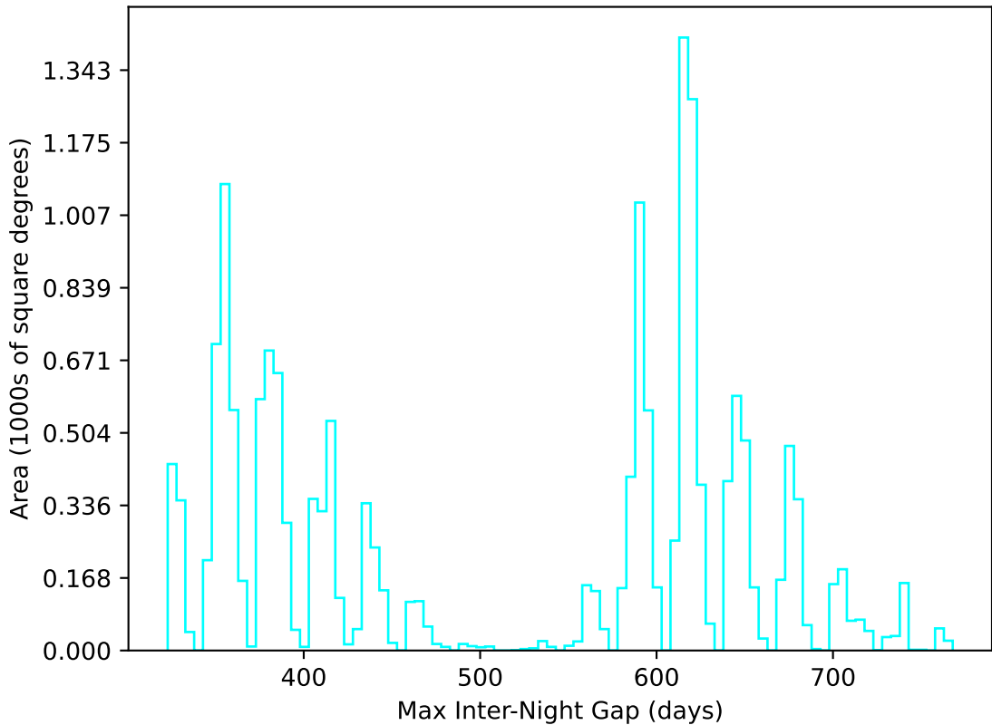
ddf_acor_sf30_lsf40_lsr20_v3.4_10yrs WFD u band: Max Inter-Night Gap
