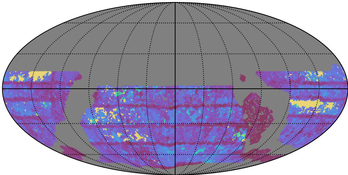
ddf_acor_sf30_lsf40_lsr20_v3.4_10yrs WFD r band: Max Inter-Night Gap
