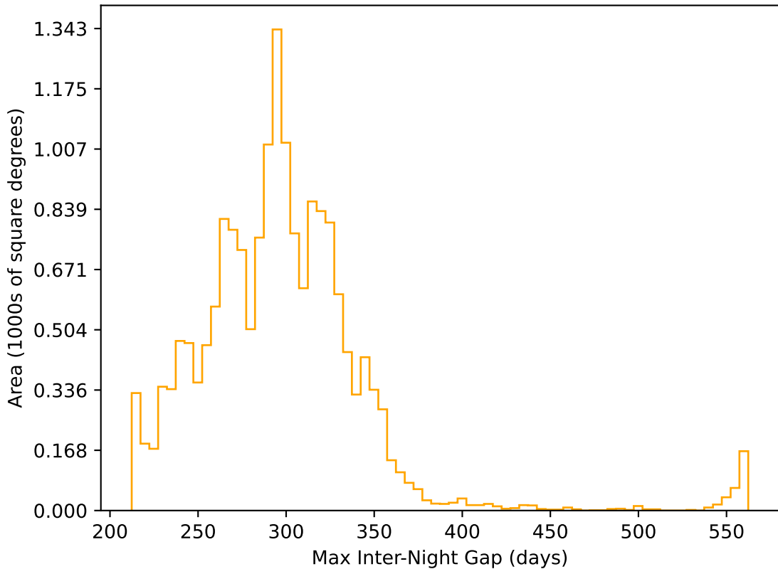
ddf_acor_sf30_lsf40_lsr20_v3.4_10yrs WFD r band: Max Inter-Night Gap
