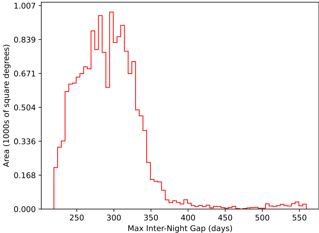
ddf_acor_sf30_lsf40_lsr20_v3.4_10yrs WFD i band: Max Inter-Night Gap
