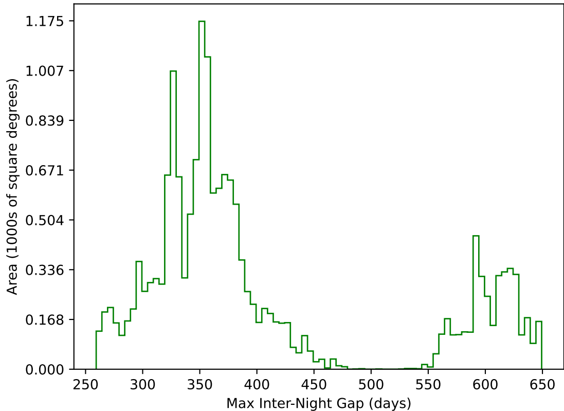
ddf_acor_sf30_lsf40_lsr20_v3.4_10yrs WFD g band: Max Inter-Night Gap
