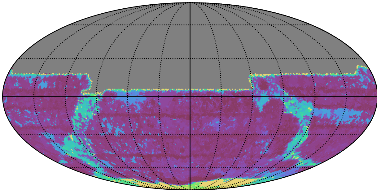
ddf_acor_sf30_lsf40_lsr20_v3.4_10yrs All sky y band: Max Inter-Night Gap
