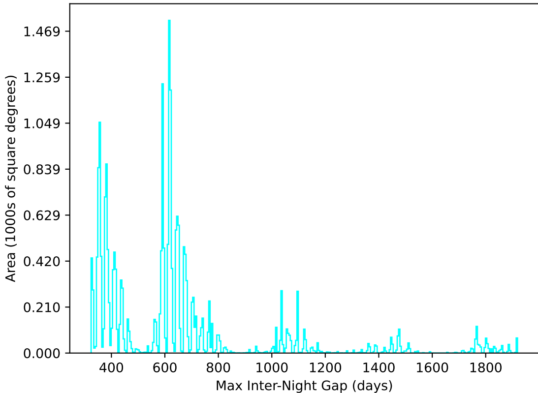
ddf_acor_sf30_lsf40_lsr20_v3.4_10yrs All sky u band: Max Inter-Night Gap
