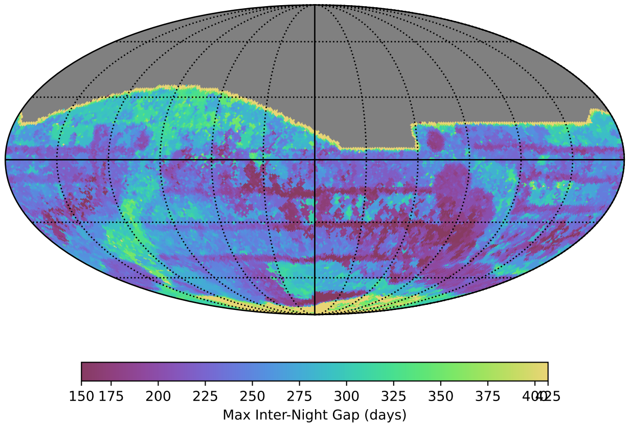
ddf_acor_sf30_lsf40_lsr20_v3.4_10yrs All sky all bands: Max Inter-Night Gap
