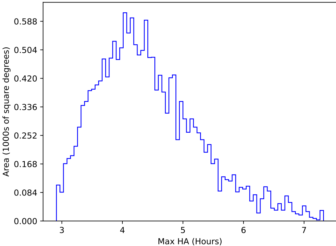
ddf_acor_sf30_lsf40_lsr20_v3.4_10yrs WFD r band: Max HA
