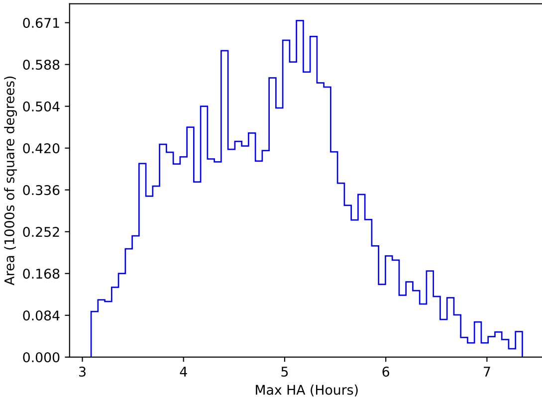
ddf_acor_sf30_lsf40_lsr20_v3.4_10yrs WFD i band: Max HA
