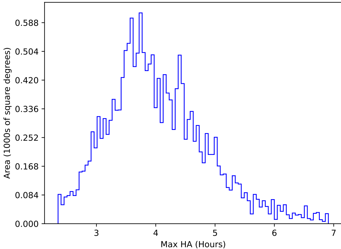
ddf_acor_sf30_lsf40_lsr20_v3.4_10yrs WFD g band: Max HA
