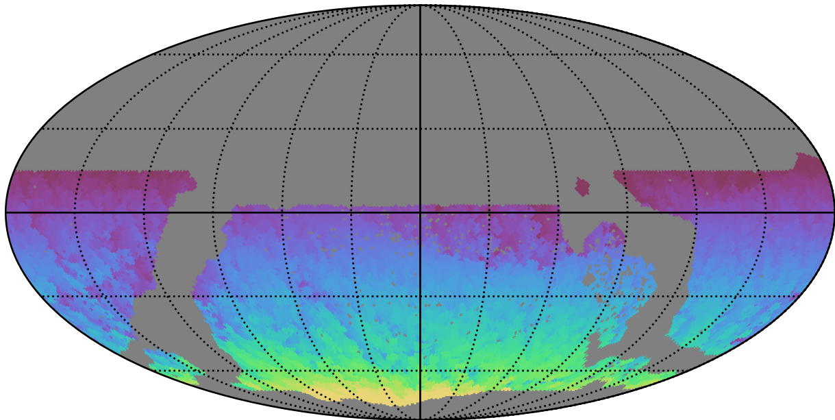
ddf_acor_sf30_lsf40_lsr20_v3.4_10yrs WFD all bands: Max HA
