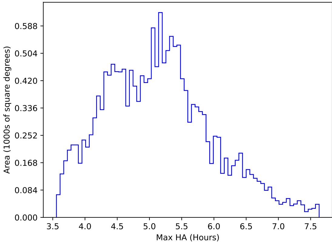
ddf_acor_sf30_lsf40_lsr20_v3.4_10yrs WFD all bands: Max HA
