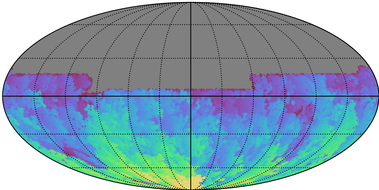
ddf_acor_sf30_lsf40_lsr20_v3.4_10yrs All sky u band: Max HA
