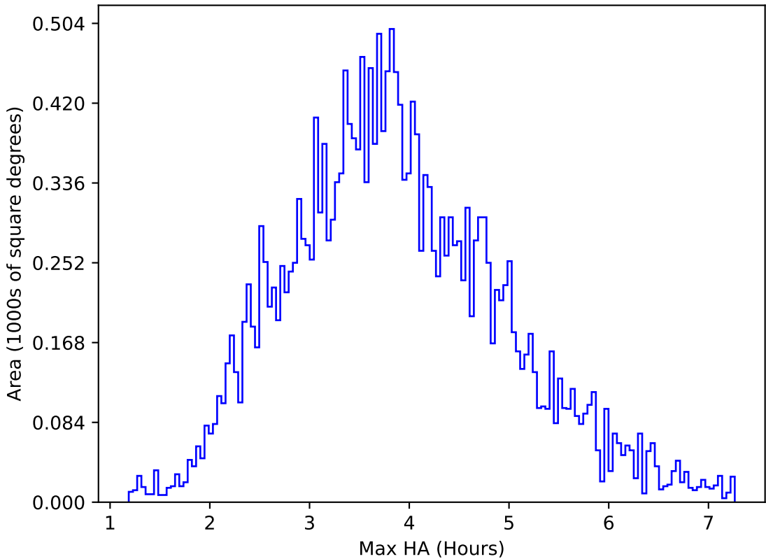
ddf_acor_sf30_lsf40_lsr20_v3.4_10yrs All sky u band: Max HA
