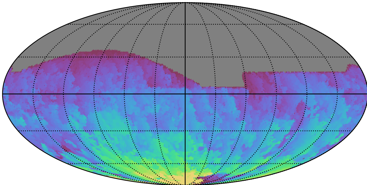
ddf_acor_sf30_lsf40_lsr20_v3.4_10yrs All sky r band: Max HA
