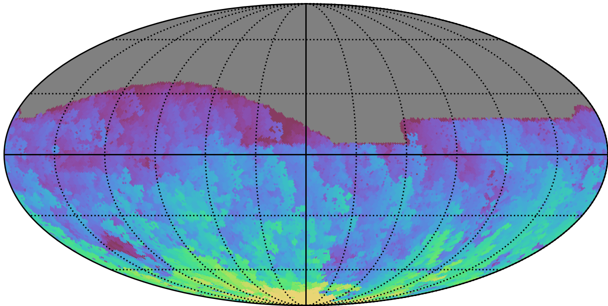
ddf_acor_sf30_lsf40_lsr20_v3.4_10yrs All sky g band: Max HA
