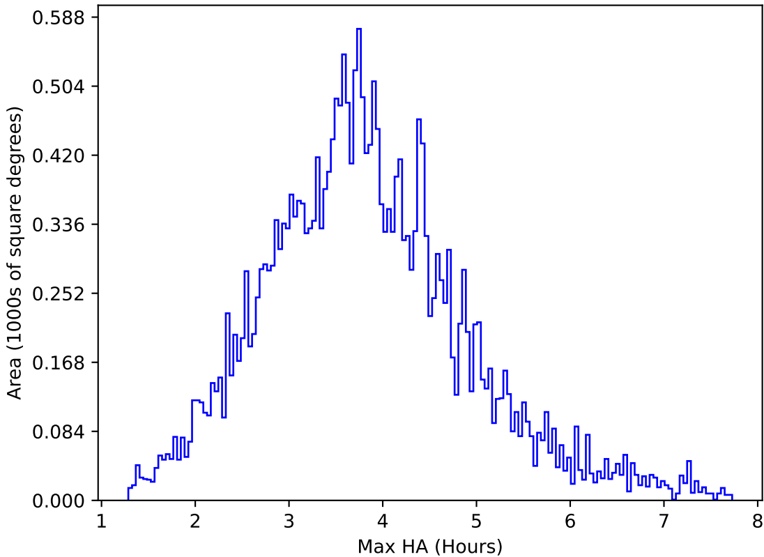
ddf_acor_sf30_lsf40_lsr20_v3.4_10yrs All sky g band: Max HA
