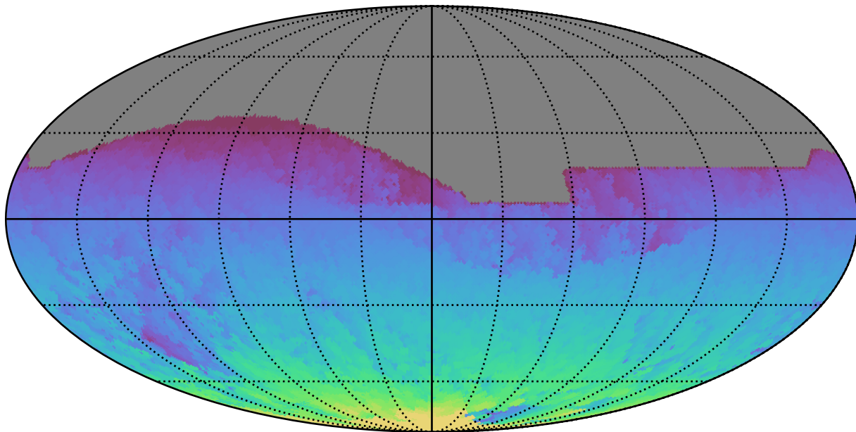
ddf_acor_sf30_lsf40_lsr20_v3.4_10yrs All sky all bands: Max HA
