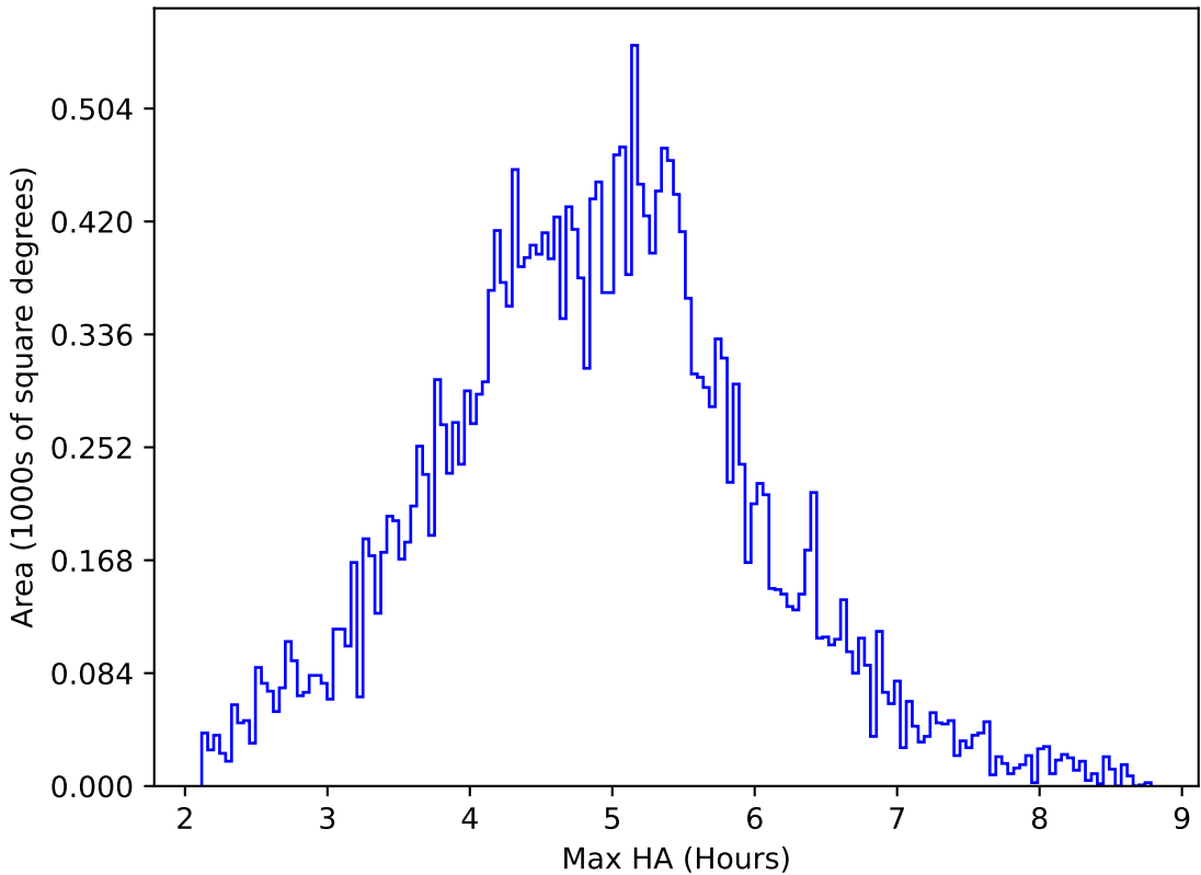
ddf_acor_sf30_lsf40_lsr20_v3.4_10yrs All sky all bands: Max HA
