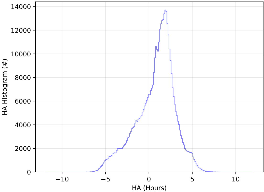
ddf_acor_sf30_lsf40_lsr20_v3.4_10yrs WFD z band: HA Histogram
