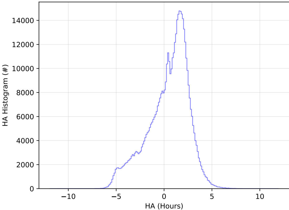
ddf_acor_sf30_lsf40_lsr20_v3.4_10yrs WFD r band: HA Histogram
