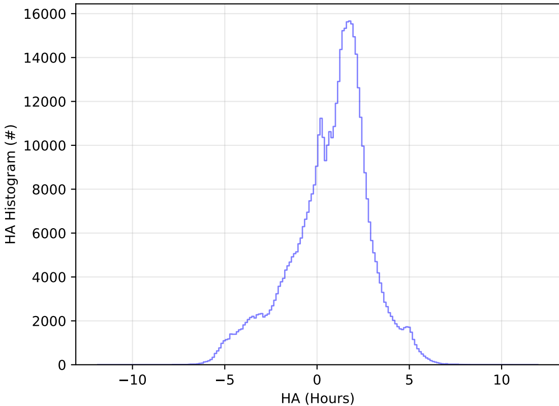
ddf_acor_sf30_lsf40_lsr20_v3.4_10yrs WFD i band: HA Histogram
