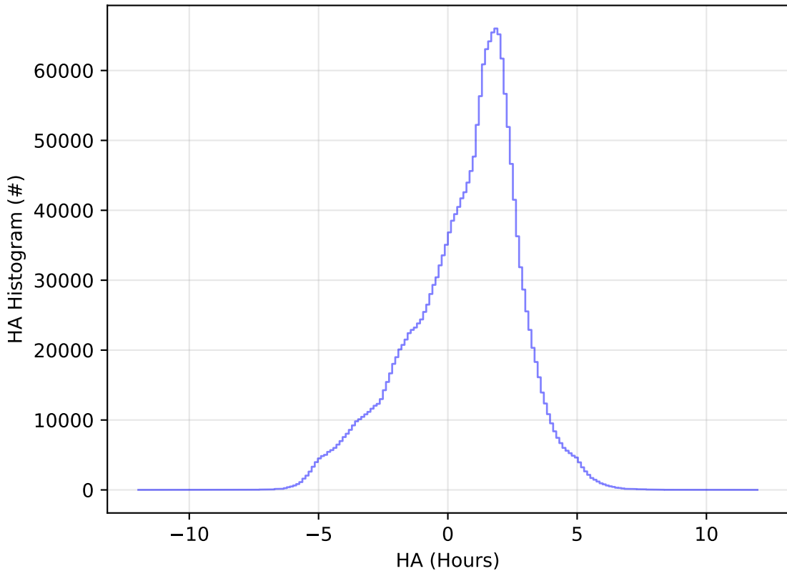
ddf_acor_sf30_lsf40_lsr20_v3.4_10yrs WFD all bands: HA Histogram
