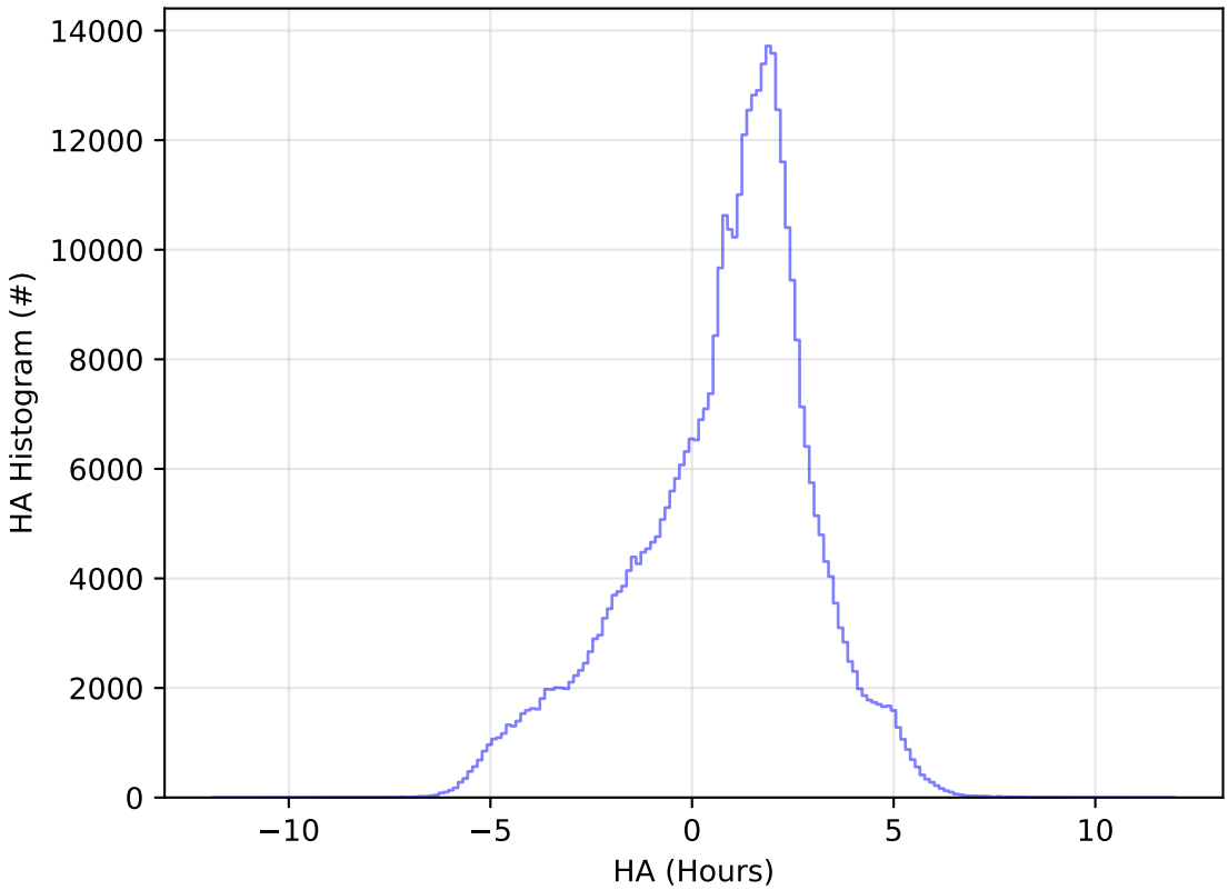
ddf_acor_sf30_lsf40_lsr20_v3.4_10yrs All sky z band: HA Histogram
