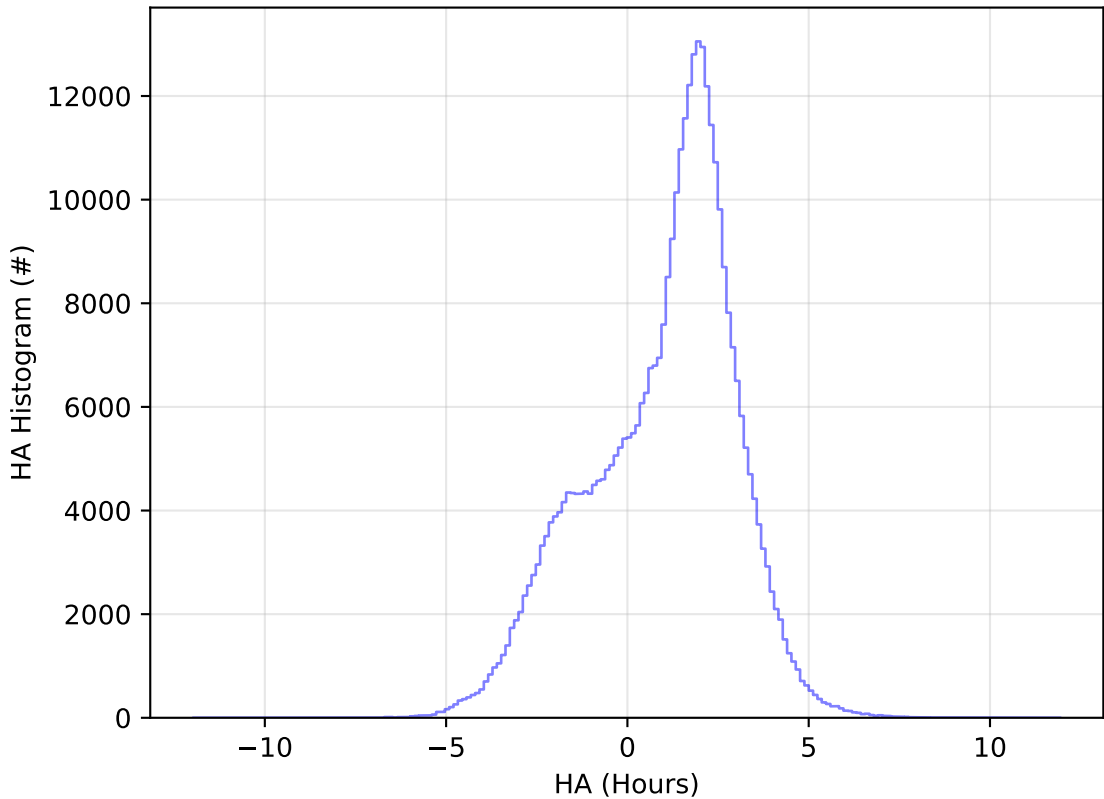
ddf_acor_sf30_lsf40_lsr20_v3.4_10yrs All sky y band: HA Histogram
