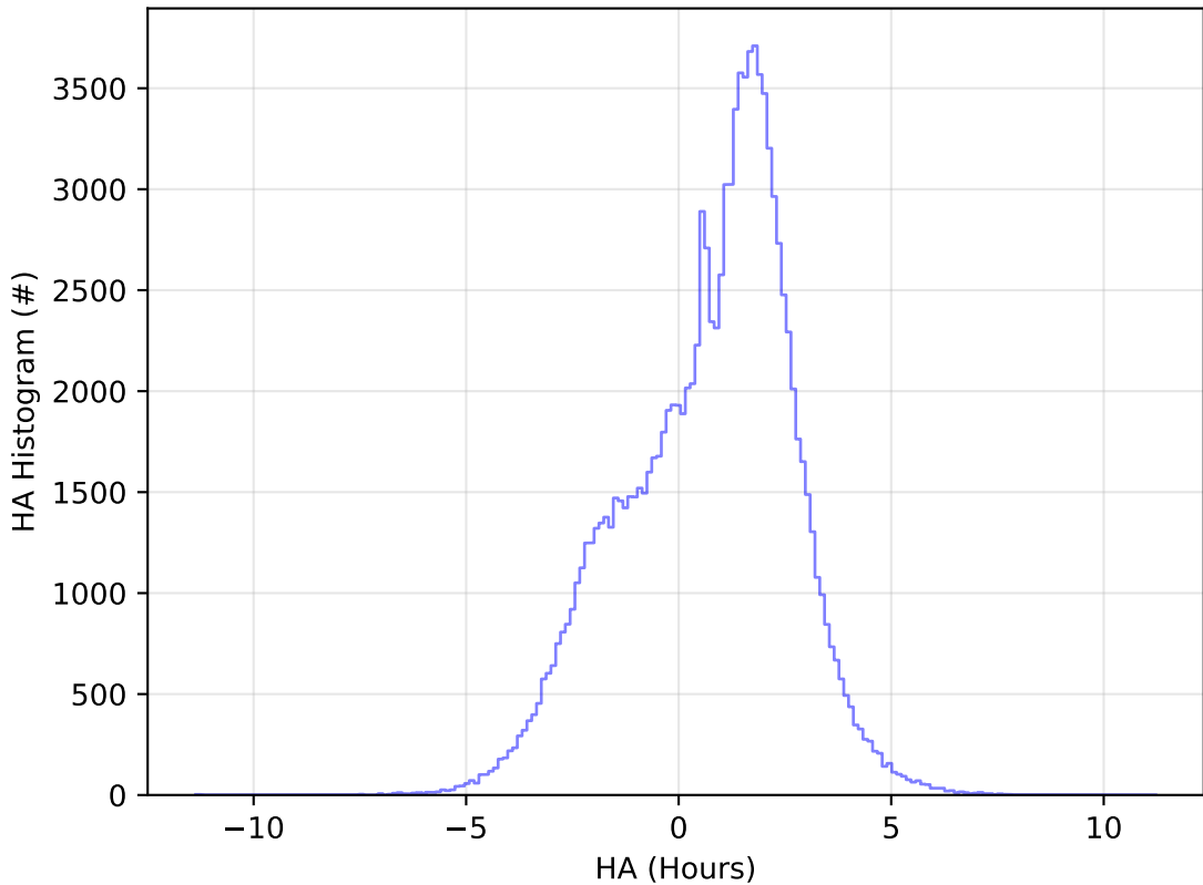
ddf_acor_sf30_lsf40_lsr20_v3.4_10yrs All sky u band: HA Histogram
