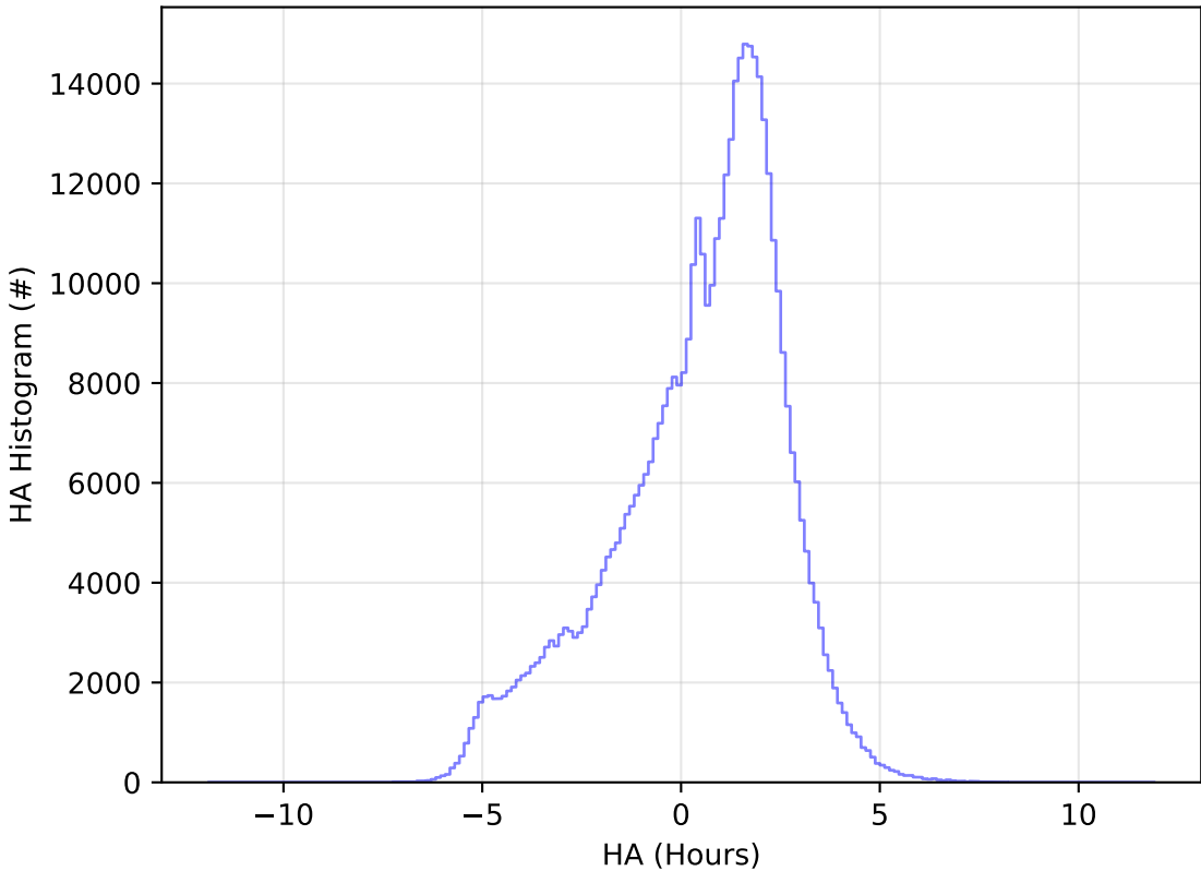
ddf_acor_sf30_lsf40_lsr20_v3.4_10yrs All sky r band: HA Histogram
