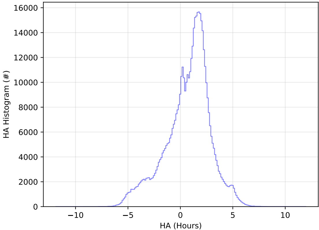
ddf_acor_sf30_lsf40_lsr20_v3.4_10yrs All sky i band: HA Histogram
