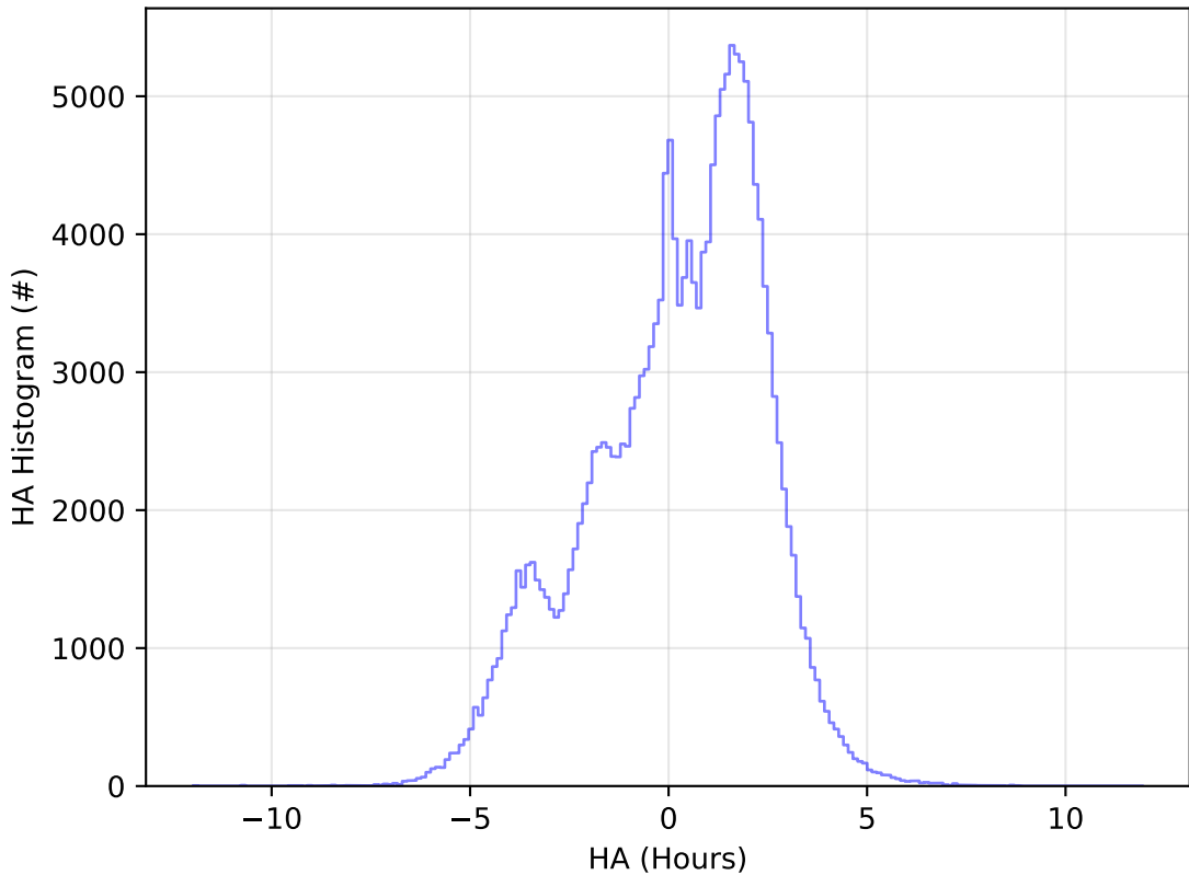
ddf_acor_sf30_lsf40_lsr20_v3.4_10yrs All sky g band: HA Histogram
