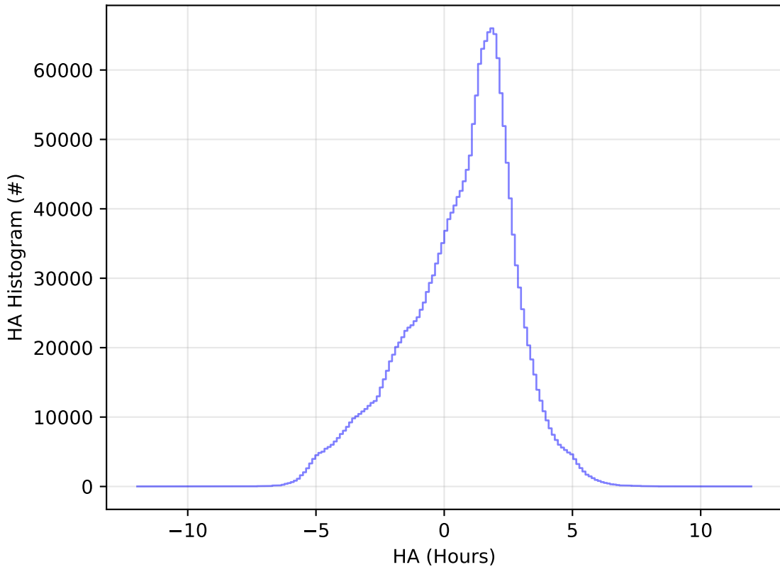
ddf_acor_sf30_lsf40_lsr20_v3.4_10yrs All sky all bands: HA Histogram
