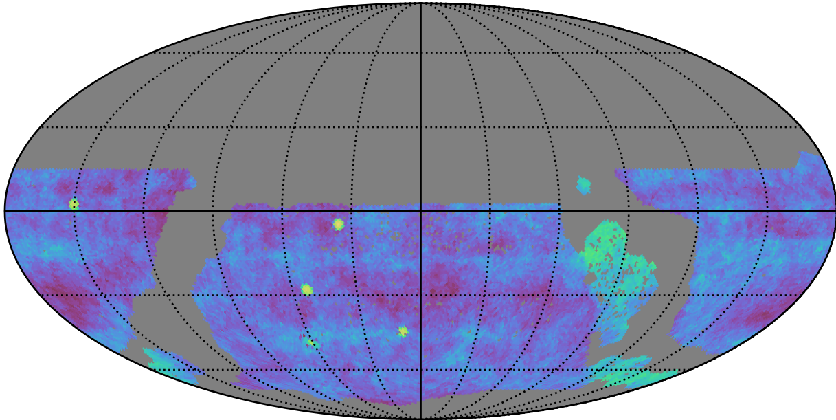
ddf_acor_sf30_lsf40_lsr20_v3.4_10yrs gri WFD: Fraction of visits in pairs (20-90 min)
