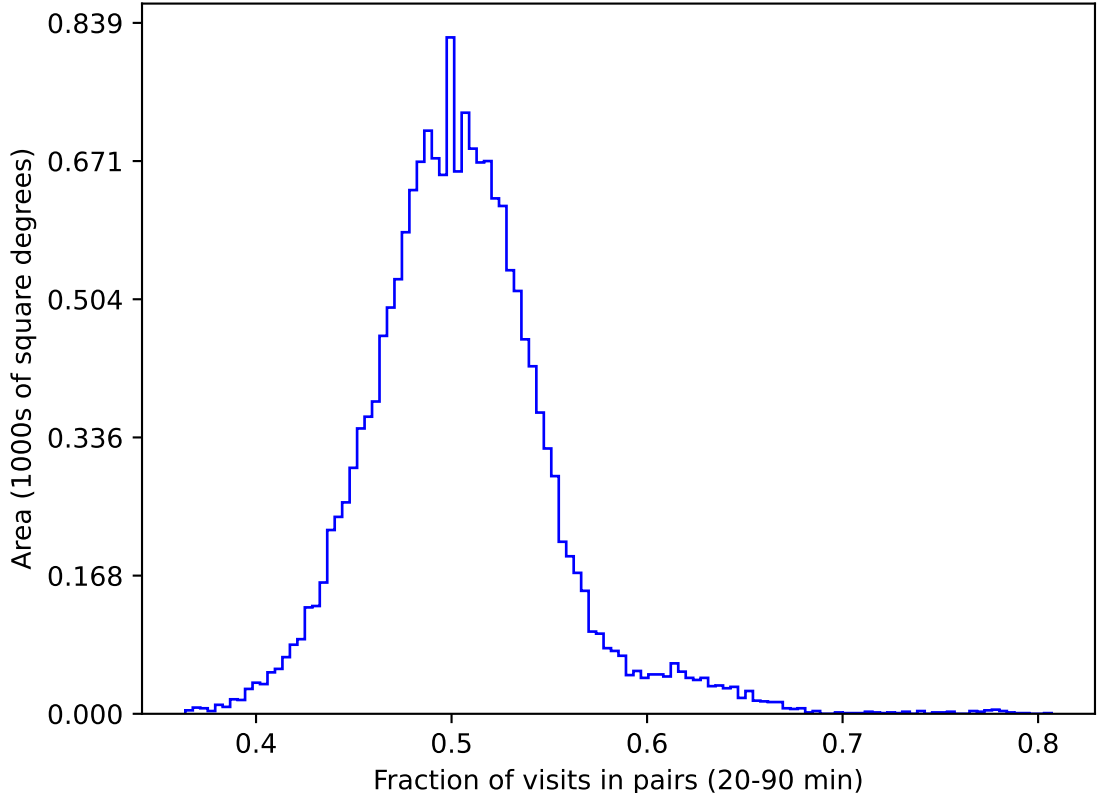
ddf_acor_sf30_lsf40_lsr20_v3.4_10yrs gri WFD: Fraction of visits in pairs (20-90 min)
