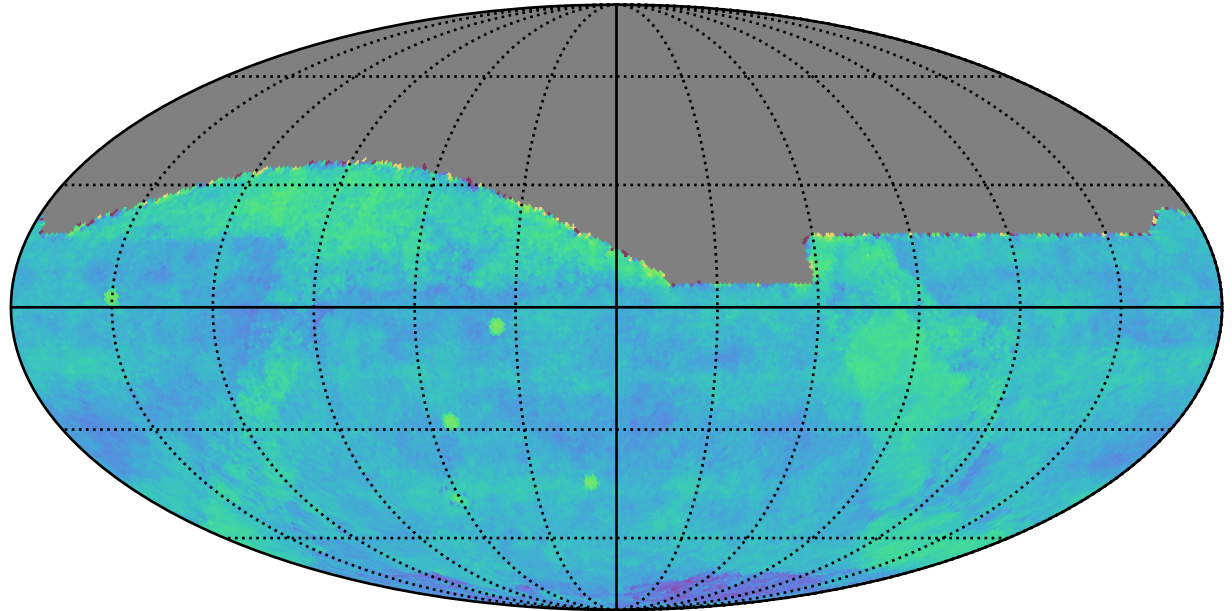
ddf_acor_sf30_lsf40_lsr20_v3.4_10yrs gri All sky: Fraction of visits in pairs (20-90 min)
