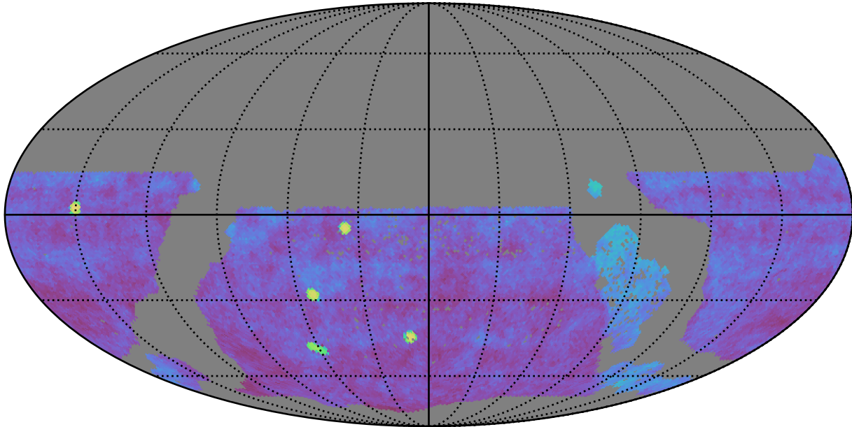
ddf_acor_sf30_lsf40_lsr20_v3.4_10yrs gri WFD: Fraction of visits in pairs (10-60 min)
