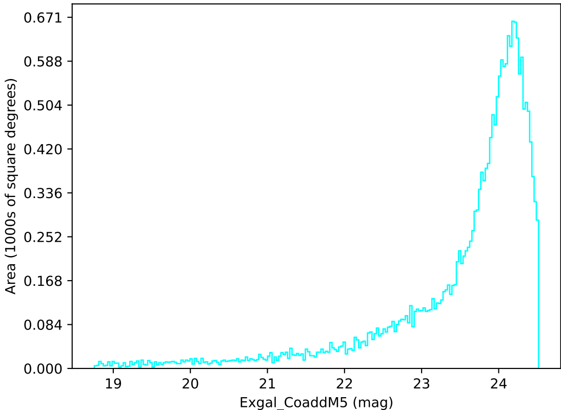
ddf_acor_sf30_lsf40_lsr20_v3.4_10yrs Yr 1 u band: Exgal_CoaddM5
