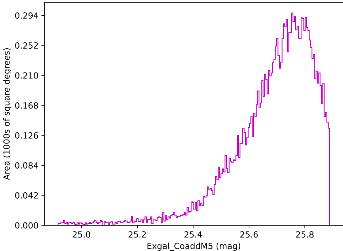
ddf_acor_sf30_lsf40_lsr20_v3.4_10yrs WFD z band: Exgal_CoaddM5
