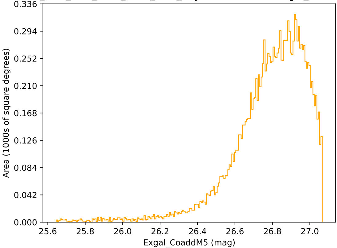
ddf_acor_sf30_lsf40_lsr20_v3.4_10yrs WFD r band: Exgal_CoaddM5
