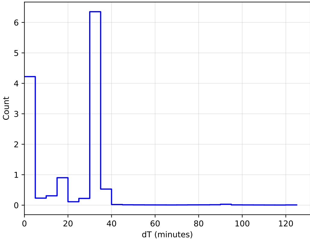
ddf_acor_sf30_lsf40_lsr20_v3.4_10yrs All sky: DeltaT Histogram
