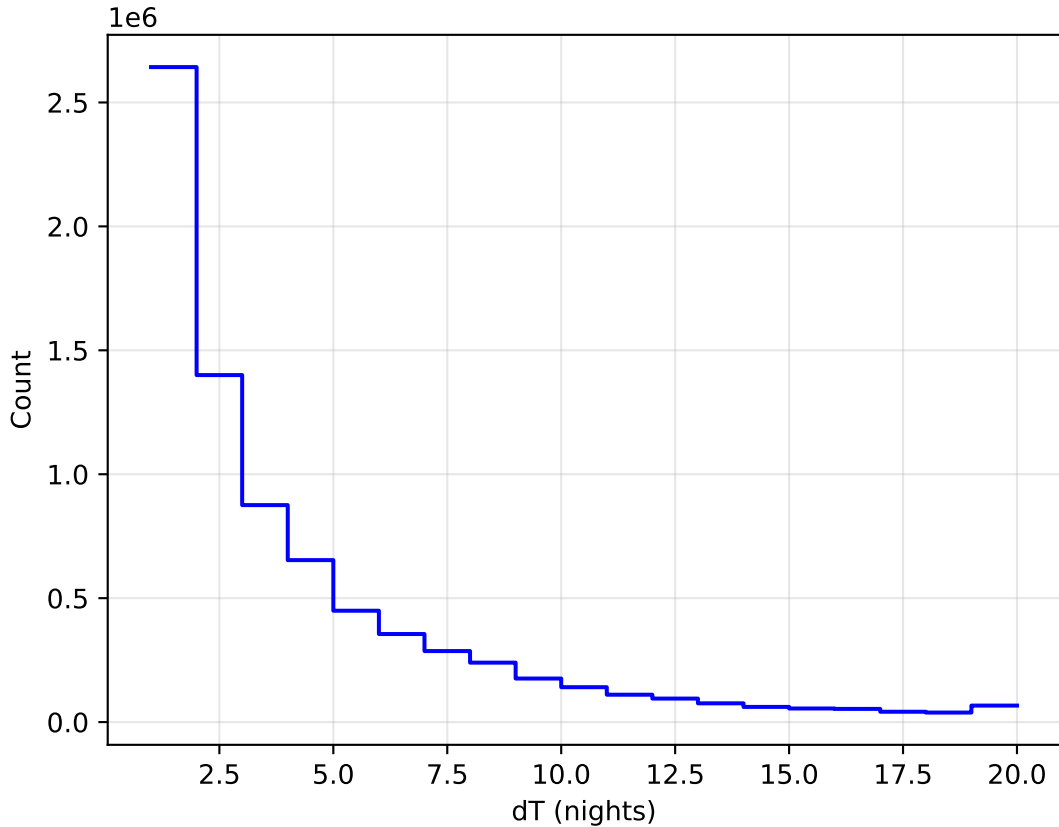
ddf_acor_sf30_lsf40_lsr20_v3.4_10yrs WFD all bands: DeltaNight Histogram
