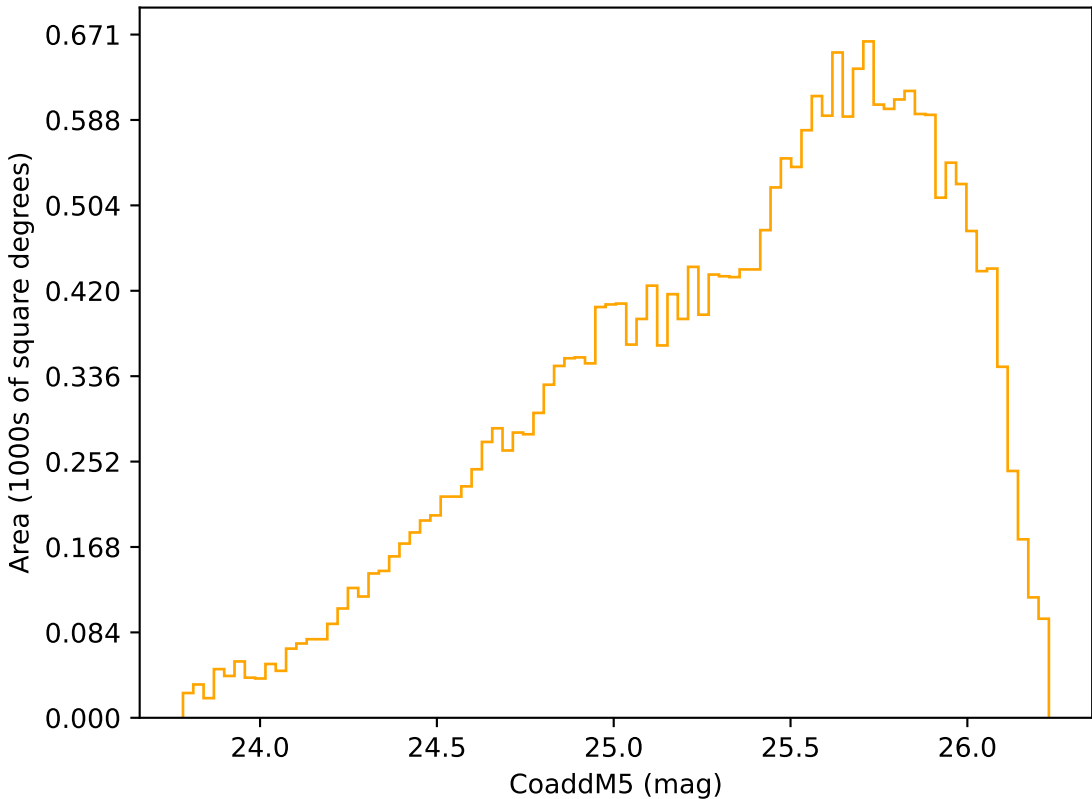
ddf_acor_sf30_lsf40_lsr20_v3.4_10yrs Yr 3-4 r band: CoaddM5
